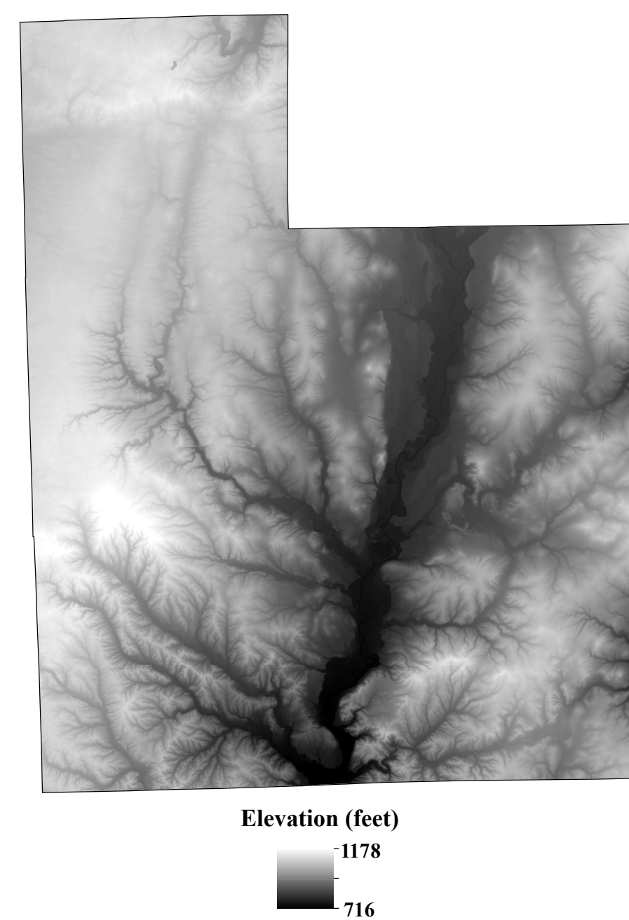
Digital Elevation Model of Fayette County, Indiana
