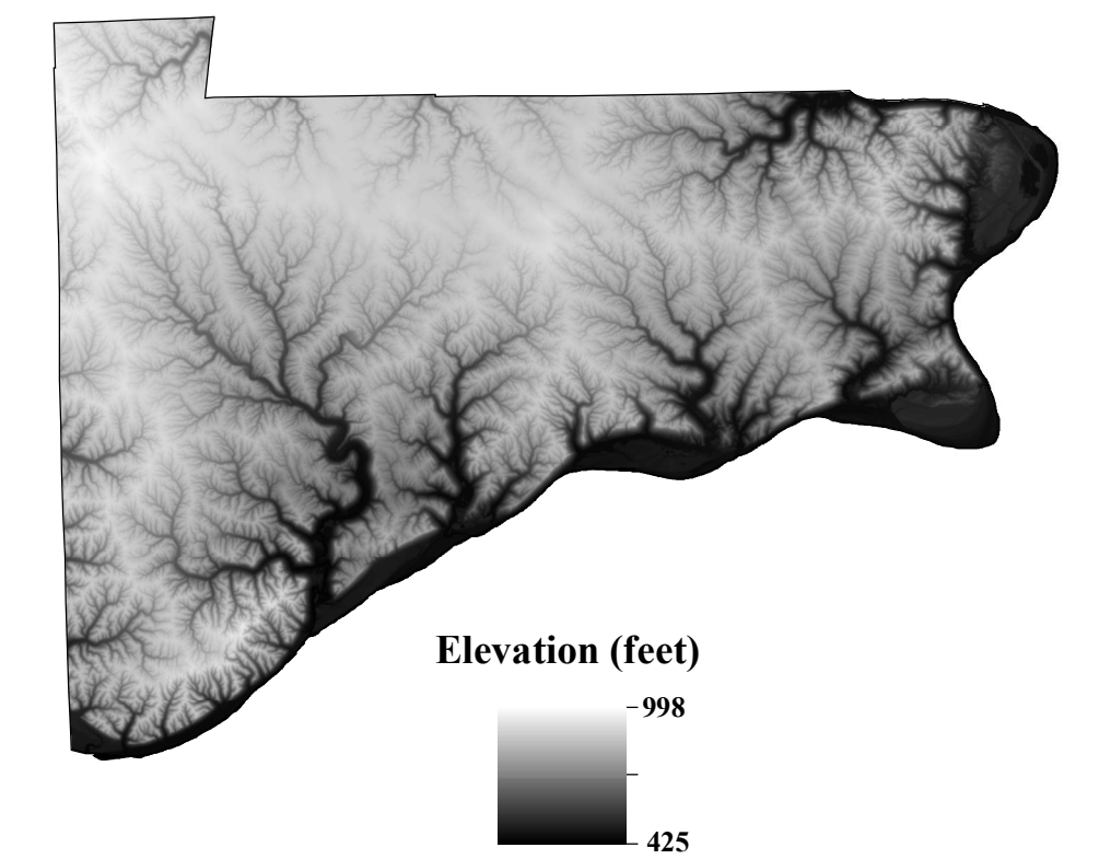
Digital Elevation Model of Switzerland County, Indiana
