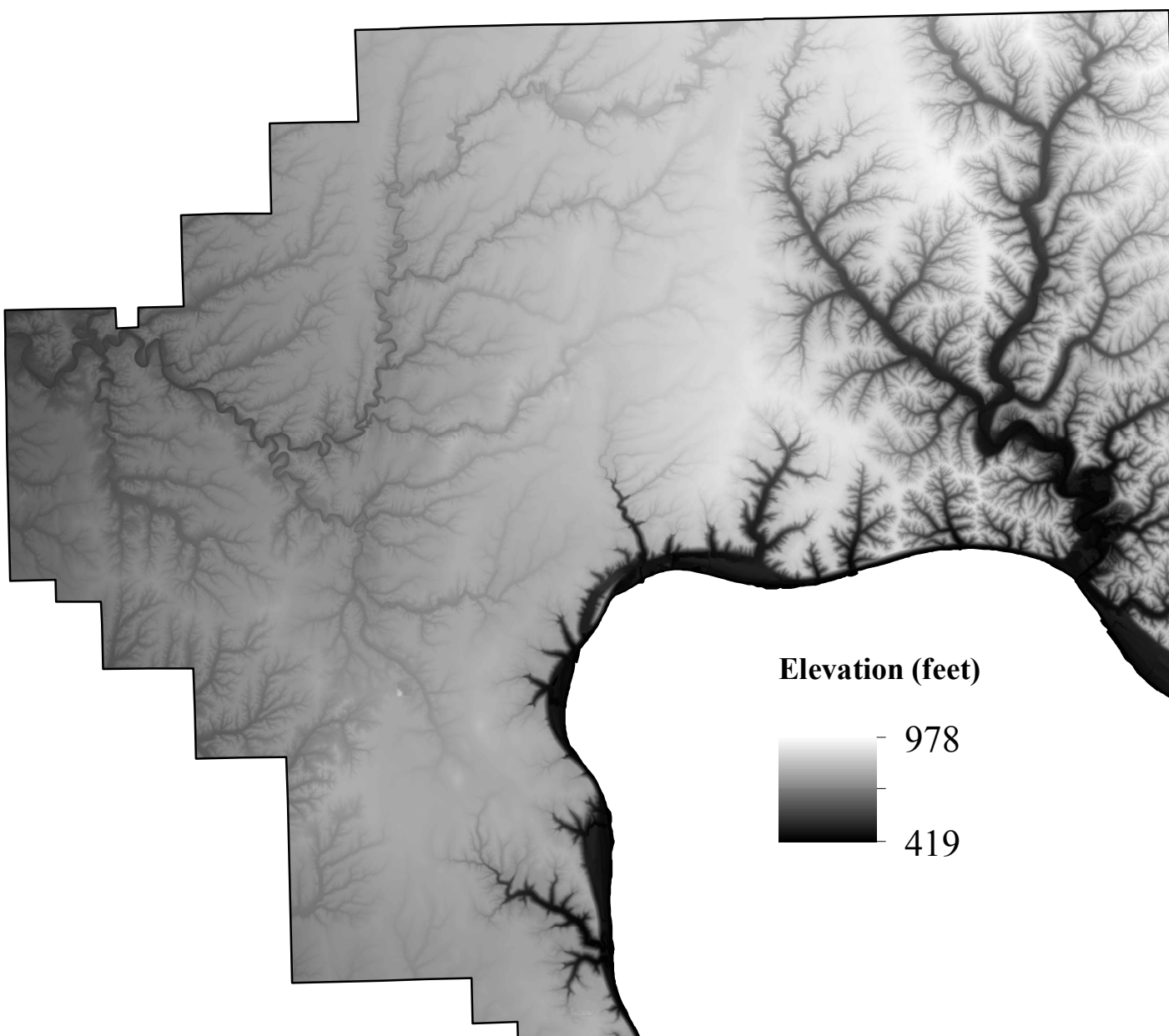
Digital Elevation Model of Jefferson County, Indiana
